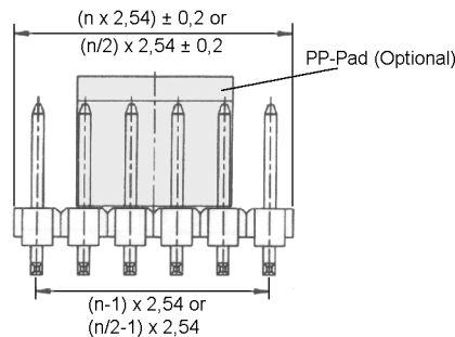
Layout B2
