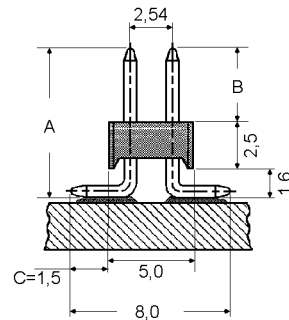
Series 3132
