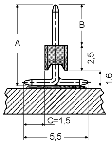
Series 3532
