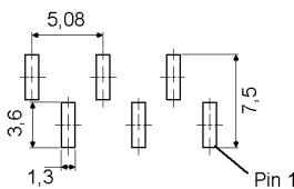
Layout B1
