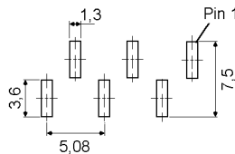
Layout B2
