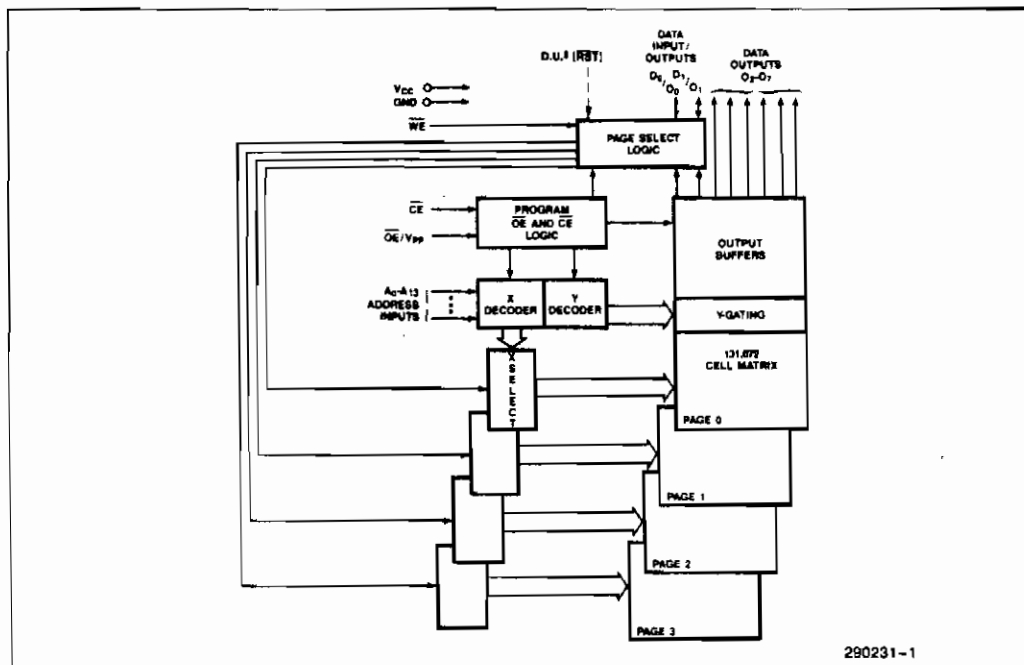
Figure 1. Block Diagram
