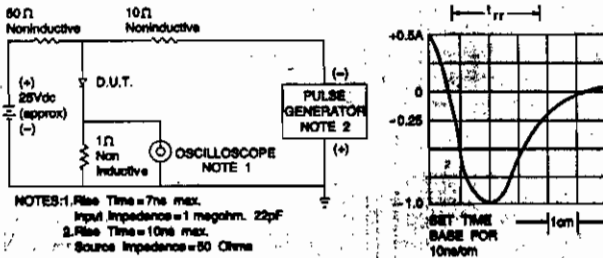
FIG. 1 - REVERSE RECOVERY TIME CHARACTERISTIC AND TEST DIAGRAM
