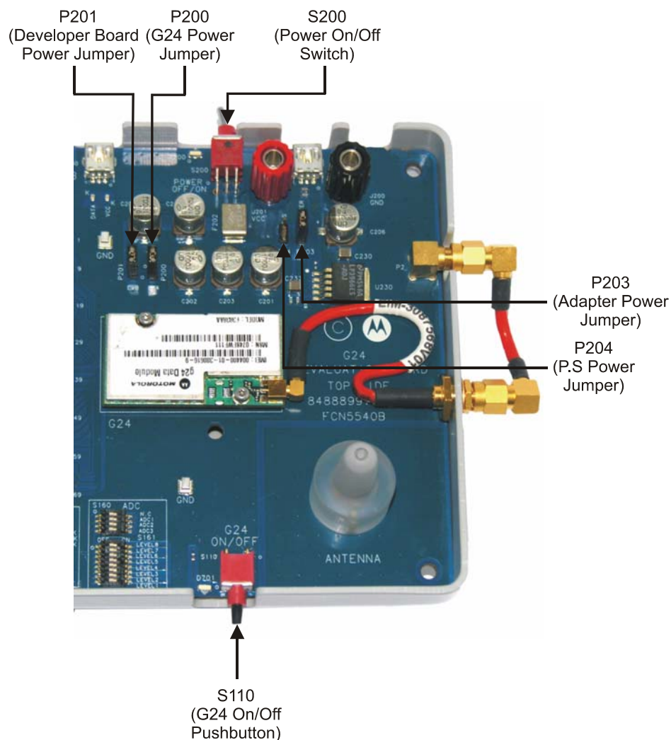
Figure 2-21: Jumpers and Switches on Developer Board
