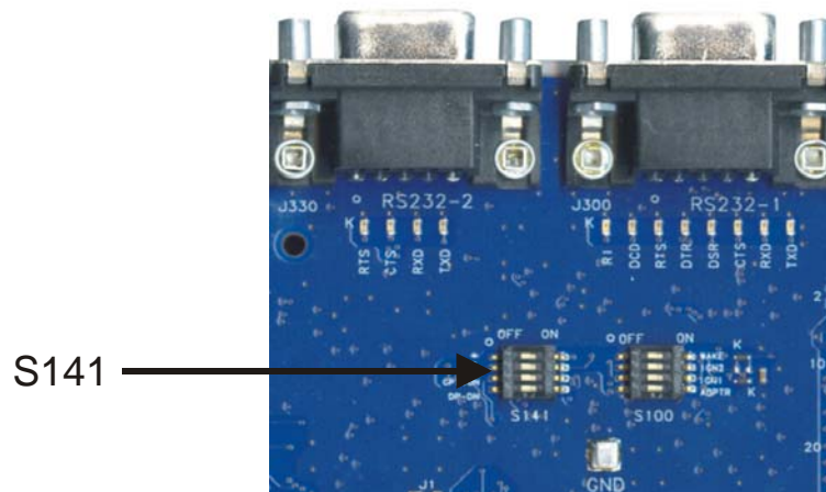
Figure 2-18: S141 Switches
