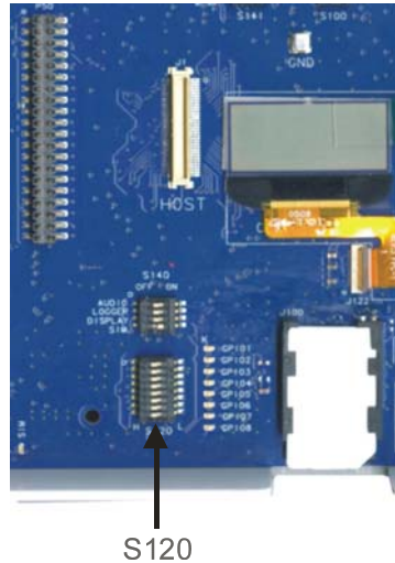
Figure 2-15: S120 Switches
