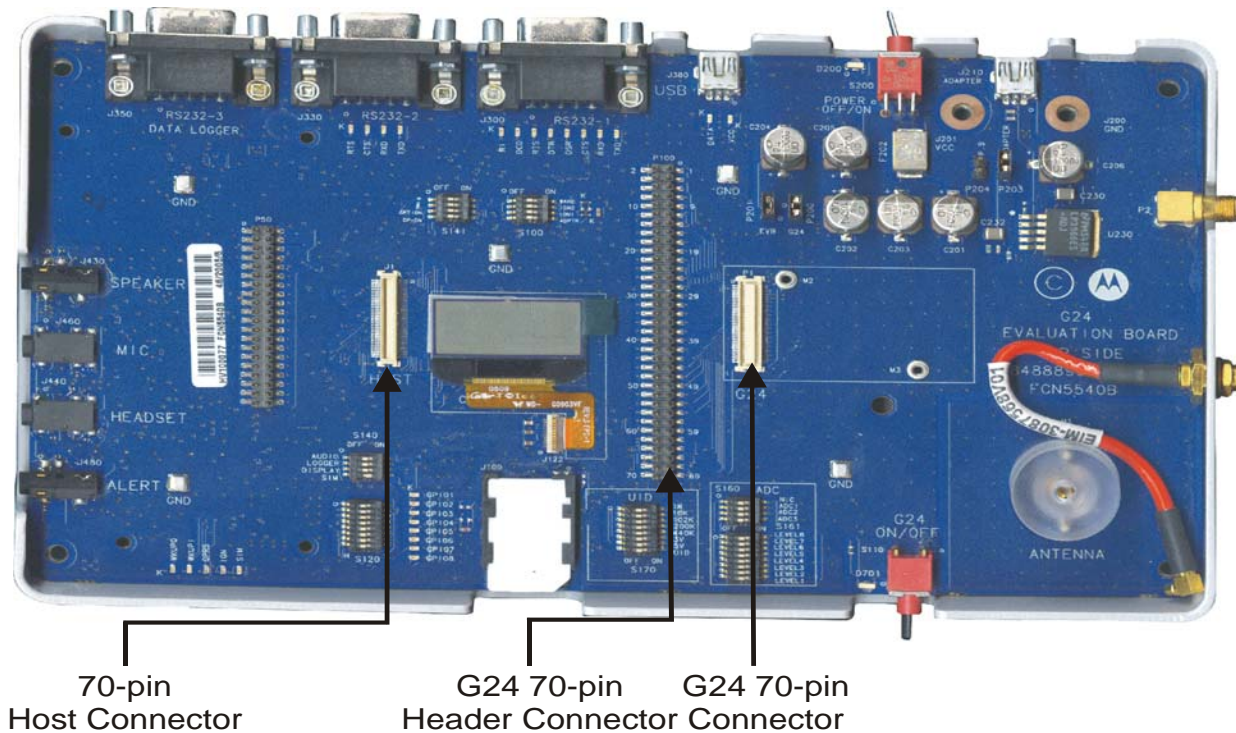
Figure 2-20: 70-pin Connectors
