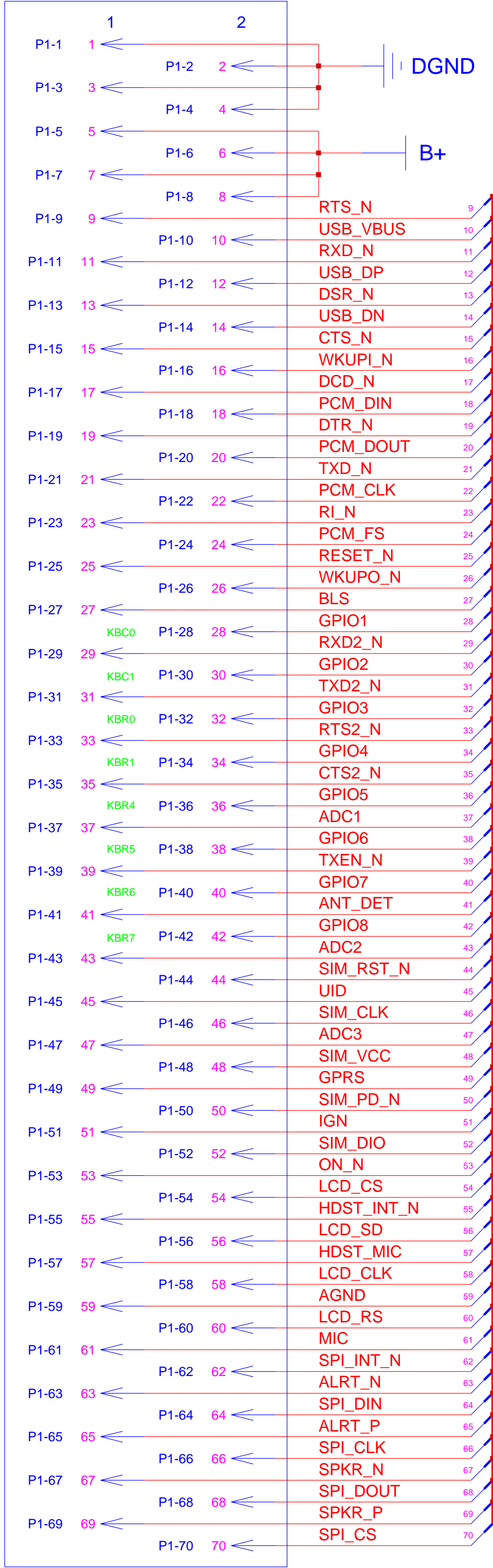
G24 70 PIN CONNECTOR (SOCKET)
