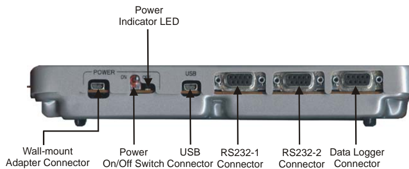
Figure 1-4: G24 Developer's Kit—Rear View with Cover
