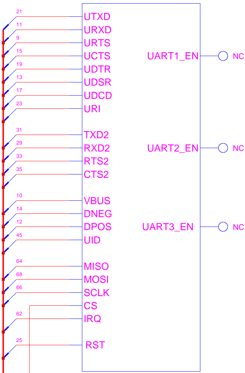
SERIAL REF# 300-399
