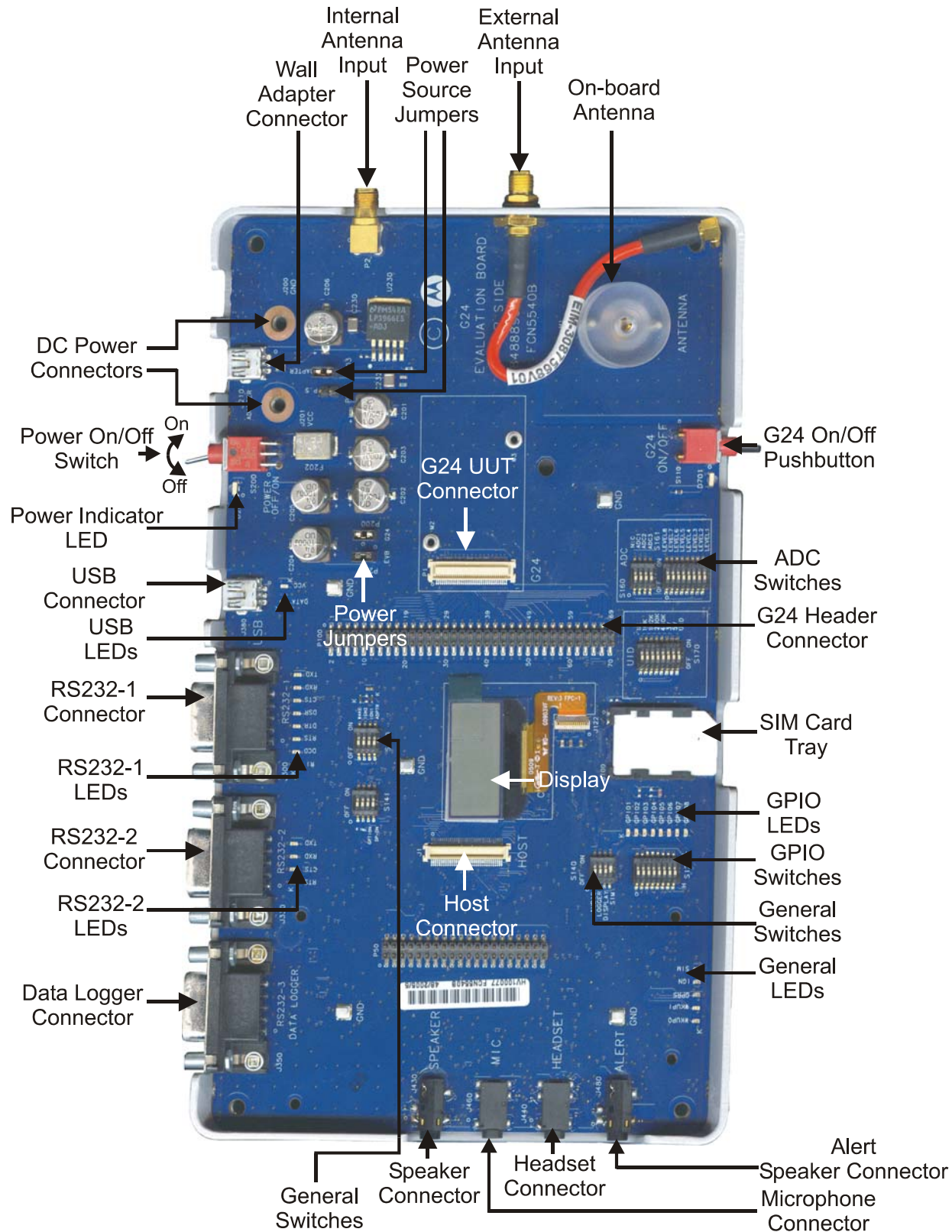
Figure 2-1: Developer Board Structure
