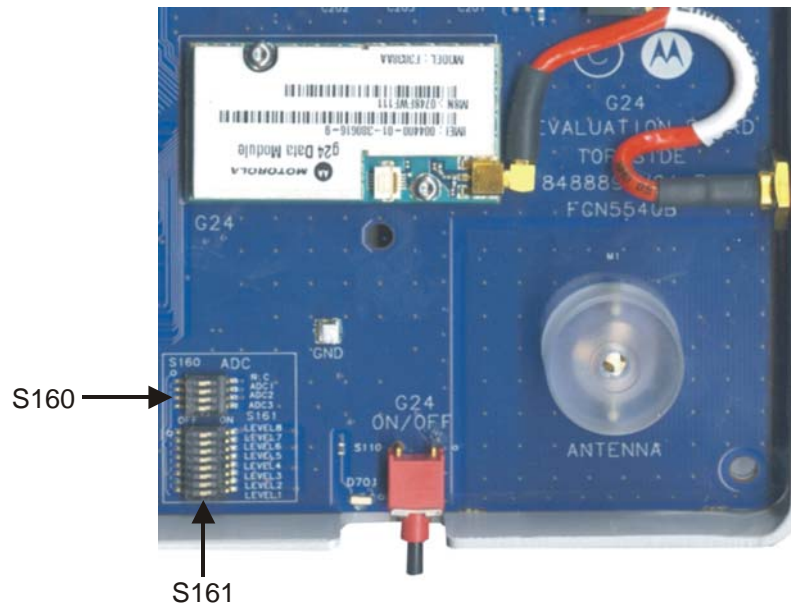
Figure 2-14: S160, S161 Switches
