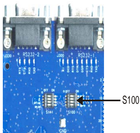
Figure 2-19: S100 Switches
