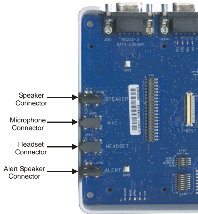
Figure 2-11: Audio Connectors
