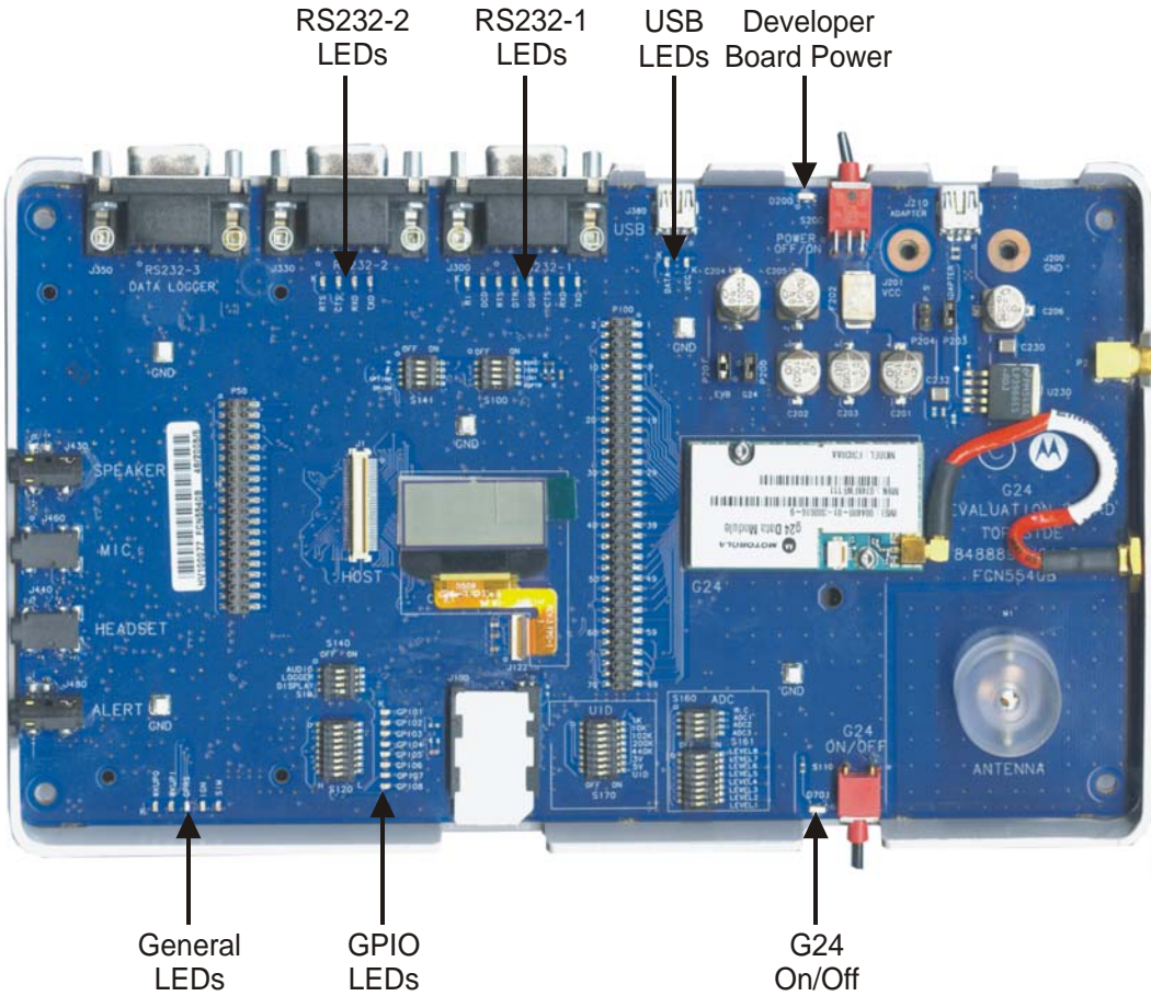
Figure 2-22: LEDs on Developer Board
