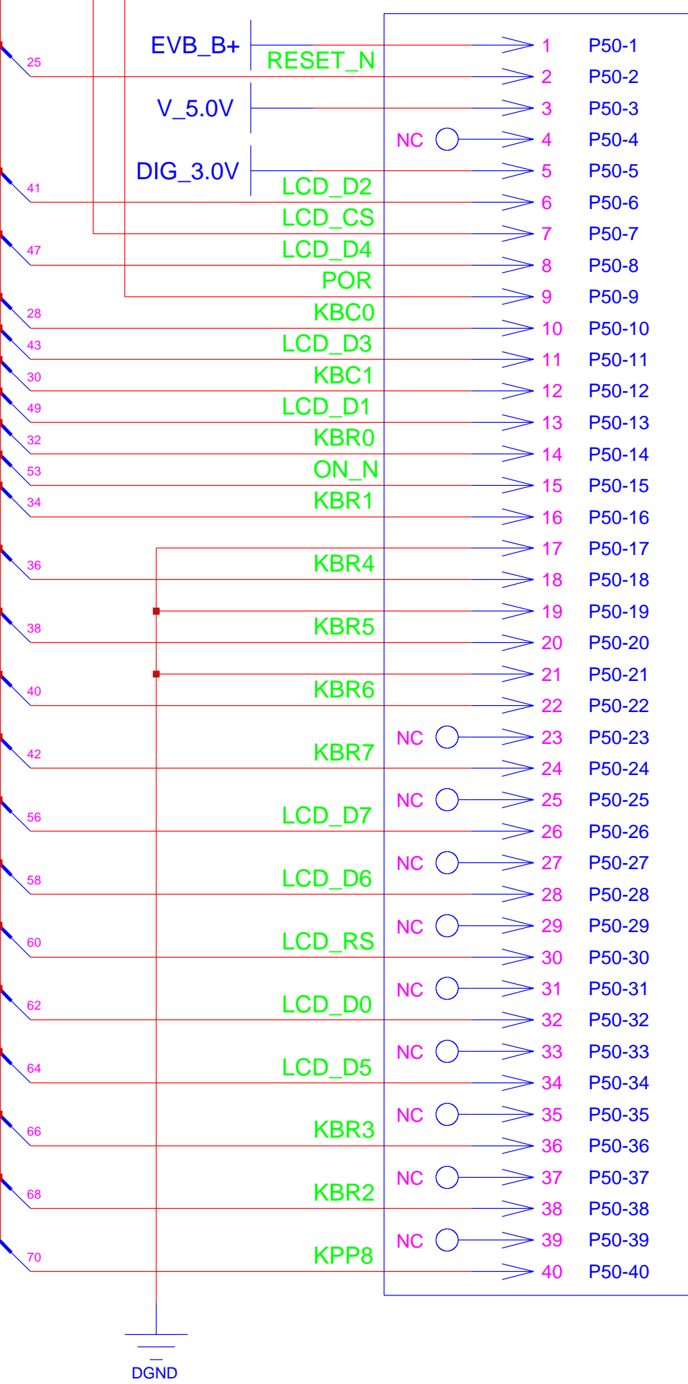
HOST 40 PIN CONNECTOR (PLUG)
