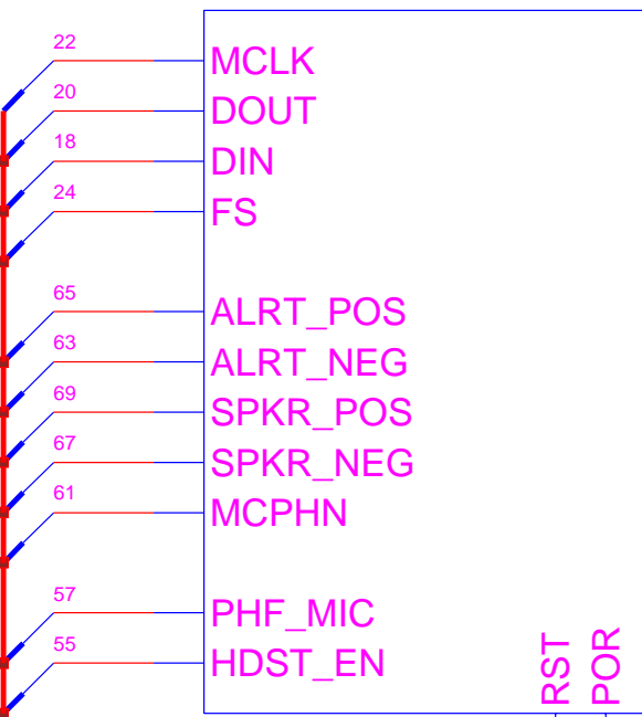
AUDIO REF# 400-499
