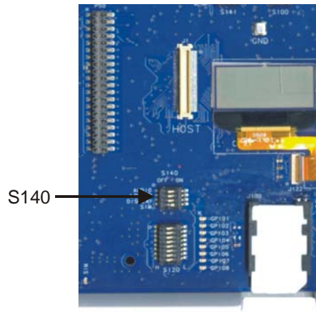
Figure 2-17: S140 Switches
