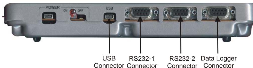
Figure 2-10: USB, RS232-1, RS232-2 and Data Logger Connectors
