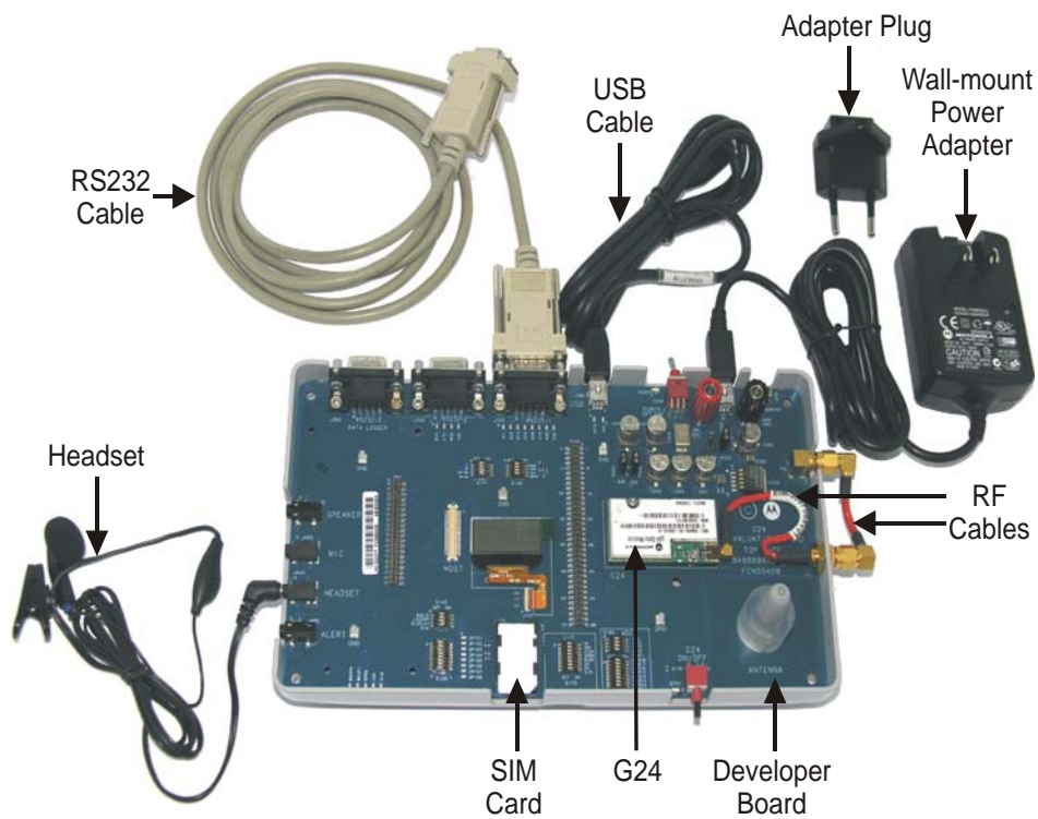
Figure 1-6: G24 Developer's Kit with Board, G24 and Accessories
