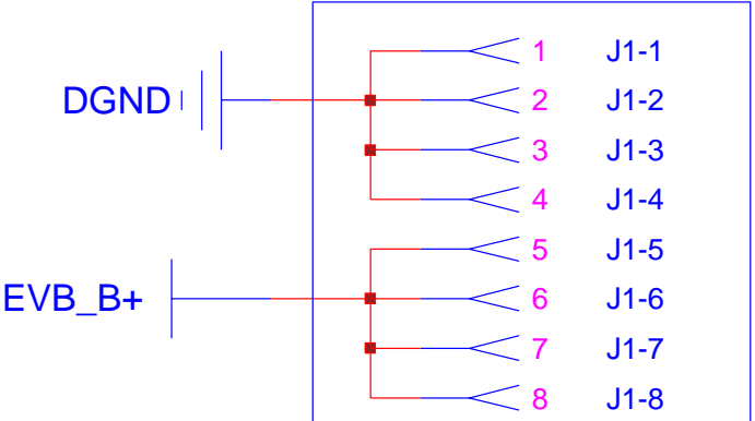
HOST 70 PIN CONNECTOR (PLUG)
