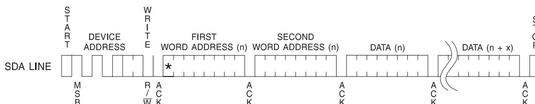
Figure 6-2. Page Write
