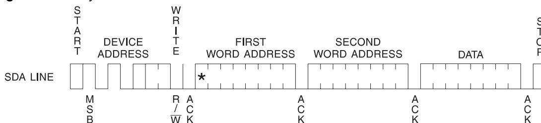
Figure 6-1. Byte Write
