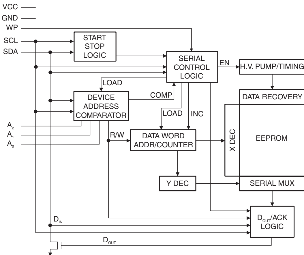
Figure 1-1. Block Diagram
