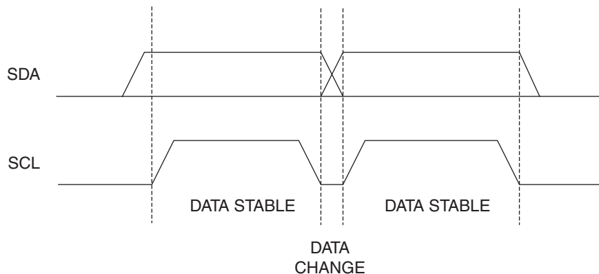
Figure 4-1. Data Validity
