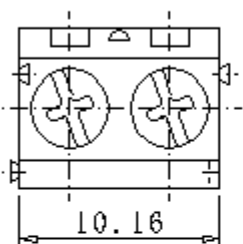
ETB33** Pitch=5.08mm
