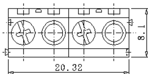
ETB33**1 Pitch=10.16mm
