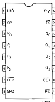
DUAL IN LINE
