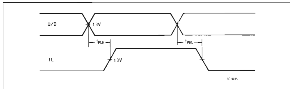
Figure 6 : Up-Down Input to Terminal Count Output Delays.
