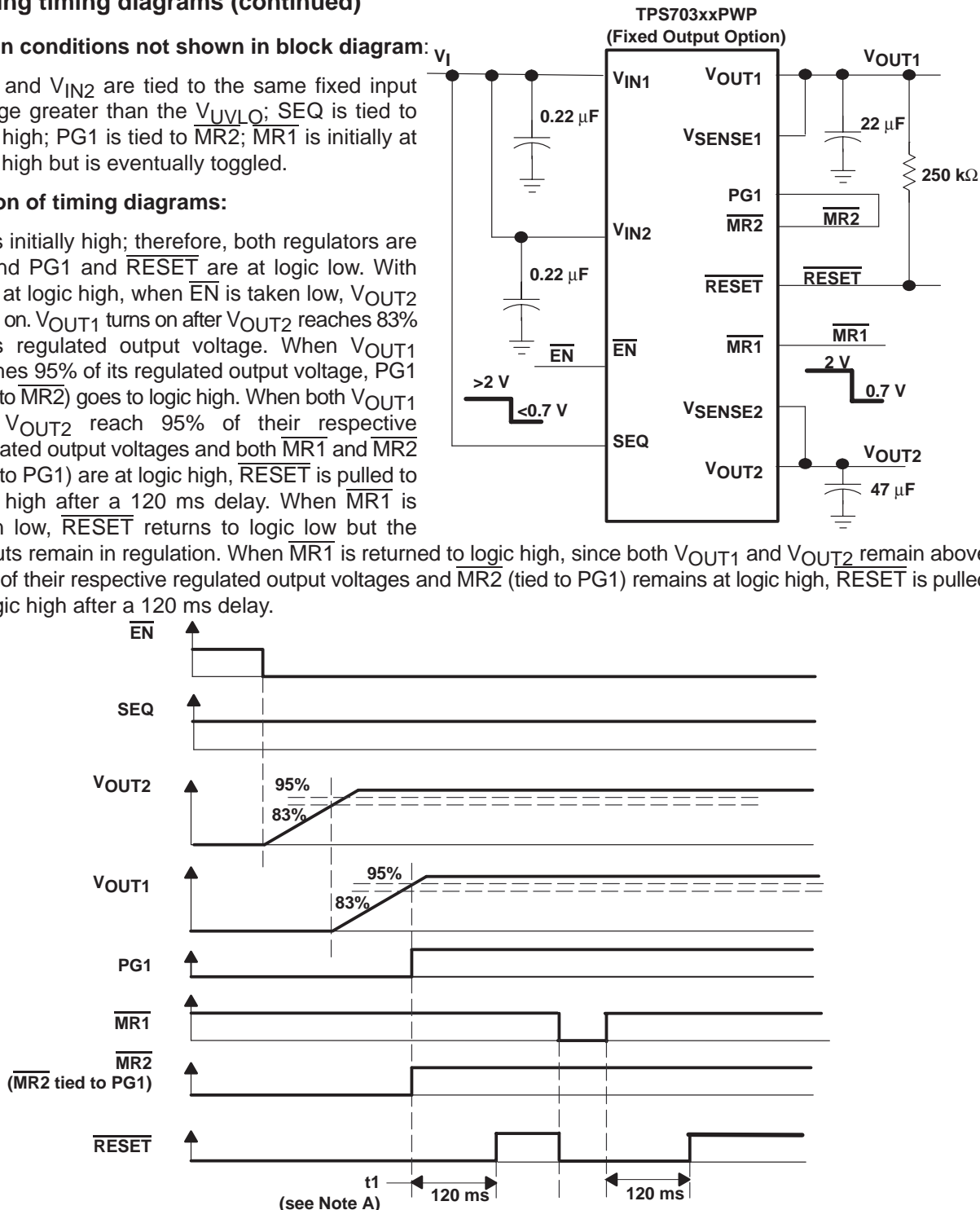
Figure 40. Timing When \overline{MR1} Is Toggled
