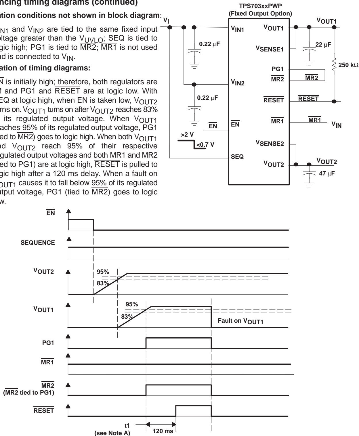
Figure 41. Timing When a Fault Occurs on V_{OUT1}
