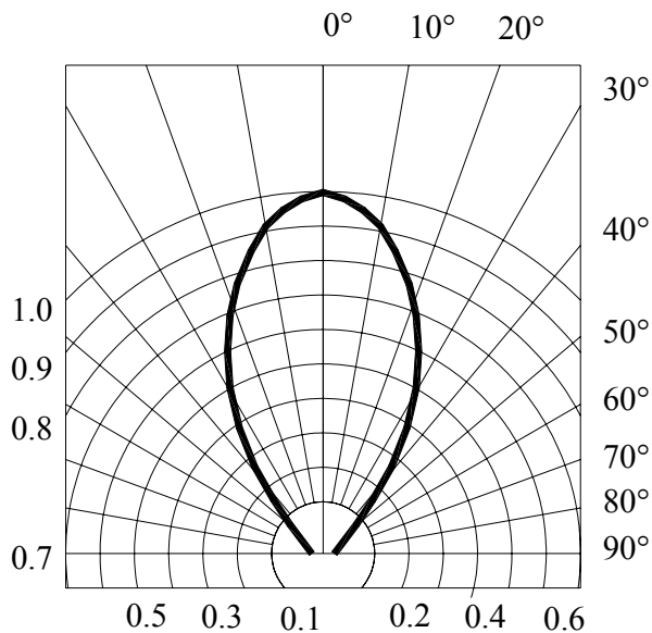
RADIATION DIAGRAM
