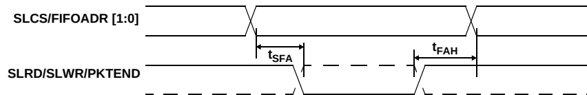
Figure 10-17. Slave FIFO Asynchronous Address Timing Diagram [20]
