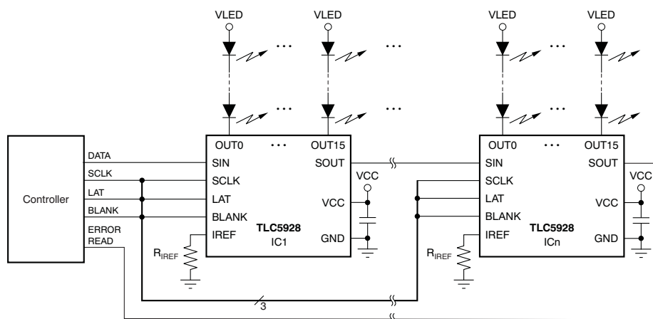
Typical Application Circuit (Multiple Daisy-Chain TLC5928s)
