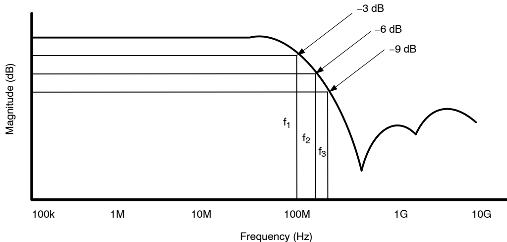
Figure 9. Filter Bandwidth
