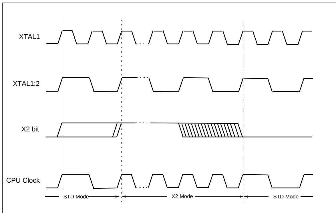
Figure 3. Mode Switching Waveforms
