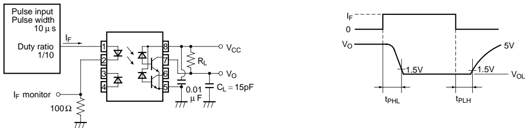
Fig. 1 Test Circuit for Propagation Delay Time
