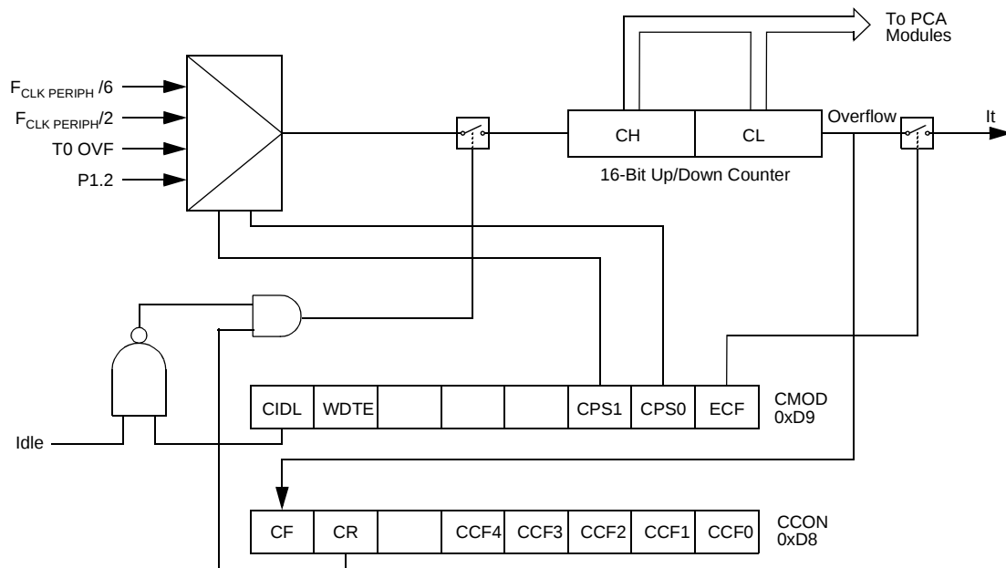
Figure 8. PCA Timer/Counter
