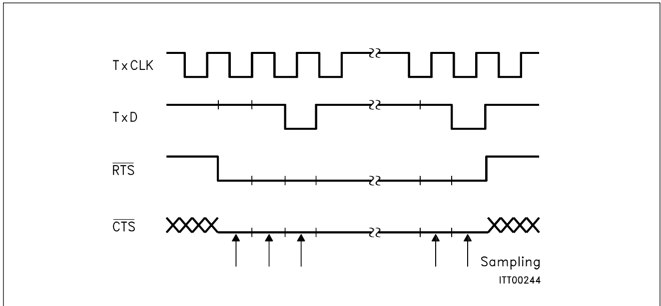
Figure 31 RTS-CTS Handshaking
