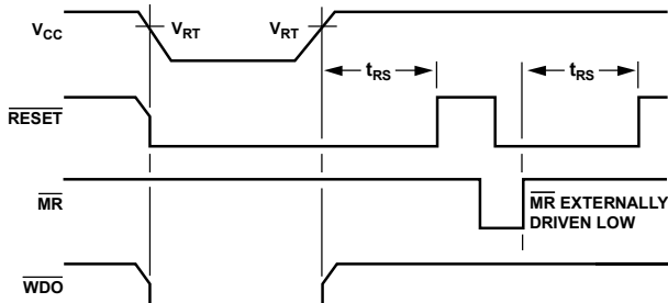
Figure 13. \overline{\text{RESET}} , \overline{\text{MR}} , and \overline{\text{WDO}} Timing
