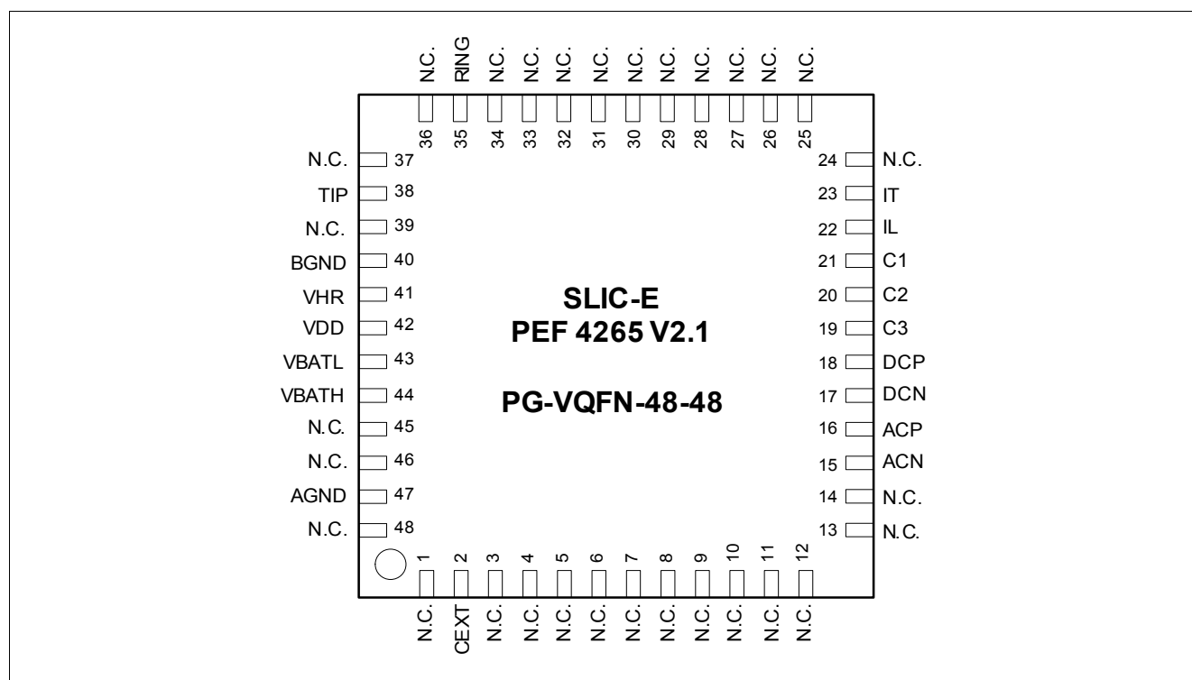
Figure 4 Pin Configuration PG-VQFN-48-48 Package (top view)
