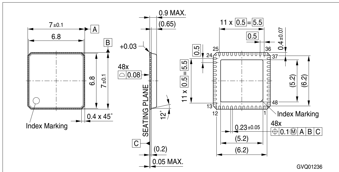
Figure 24 Package Outline for PG-VQFN-48-48 (Plastic Green Very thin Profile Quad Flatpack No-lead)
