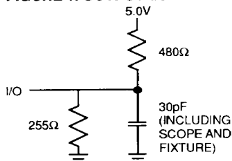
FIGURE 1. OUTPUT LOAD
