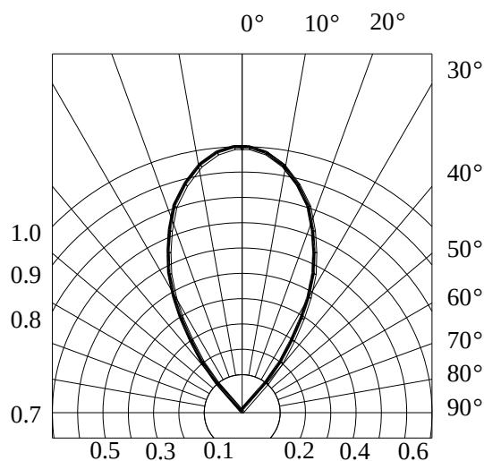
RADIATION DIAGRAM
