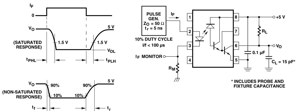
Figure 12. Switching test circuit.
