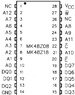
Figure 1. Pin Connections
