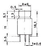
ST 1044 1-pole ST 1042 2-pole
