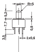
ST 1034 D 1-pole
