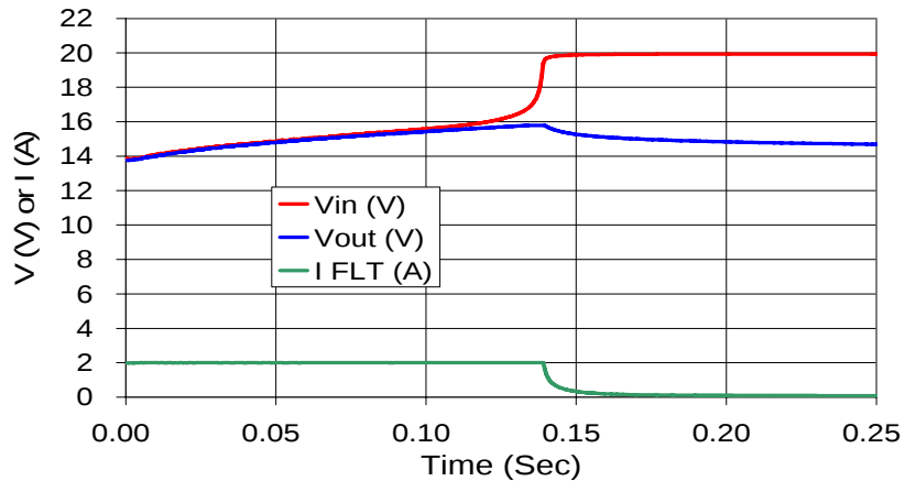
Typical Fault Response: ZEN132V230A16LS 20 V/2 A Current Limited Source ( I_{OUT}=0 )
