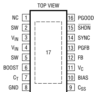
FE PACKAGE 16-LEAD PLASTIC TSSOP
