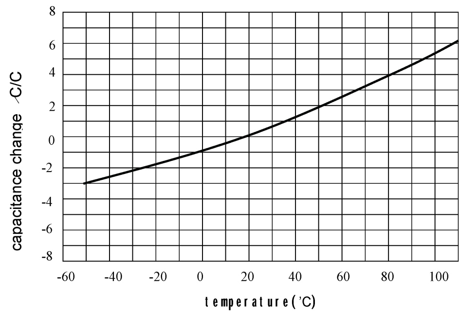
9.2 capacitance change vs temperature
