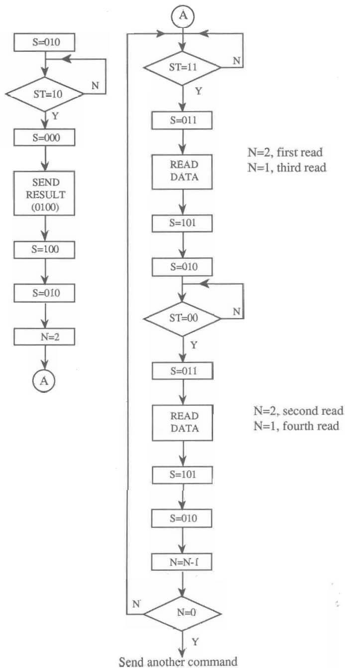
Fig 2. Control flow of the CPU mode for resulting.
