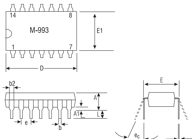
14-Pin DIP
