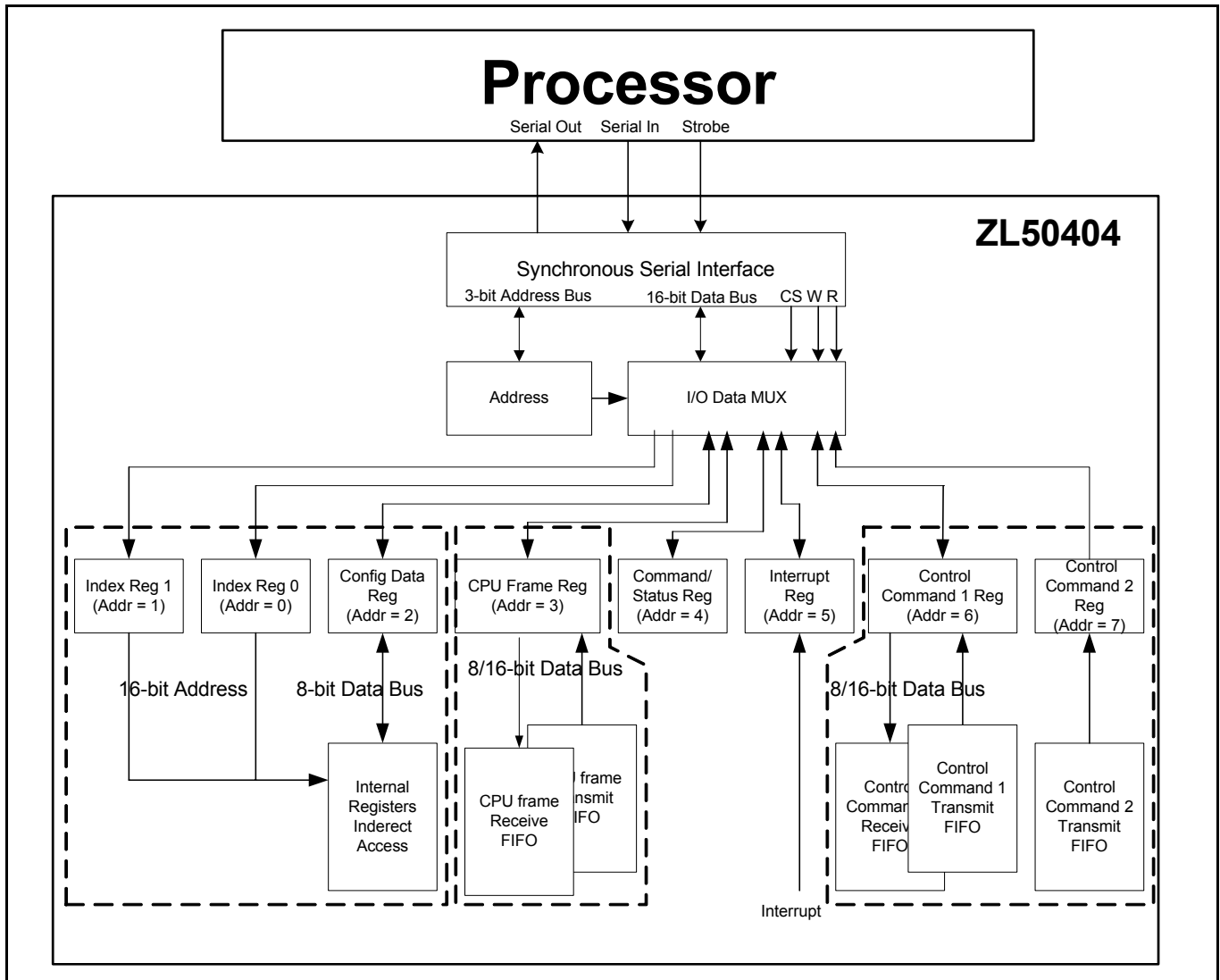
Figure 3 - Overview of the ZL50404 SSI Interface
