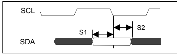
Figure 19 - I 2 C Input Setup Timing
