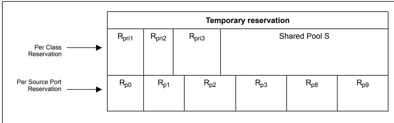
Figure 8 - Buffer Partition Scheme Used to Implement Buffer Management in the ZL50404
