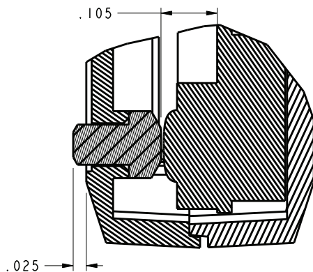
DETAIL A SCALE 4.000
