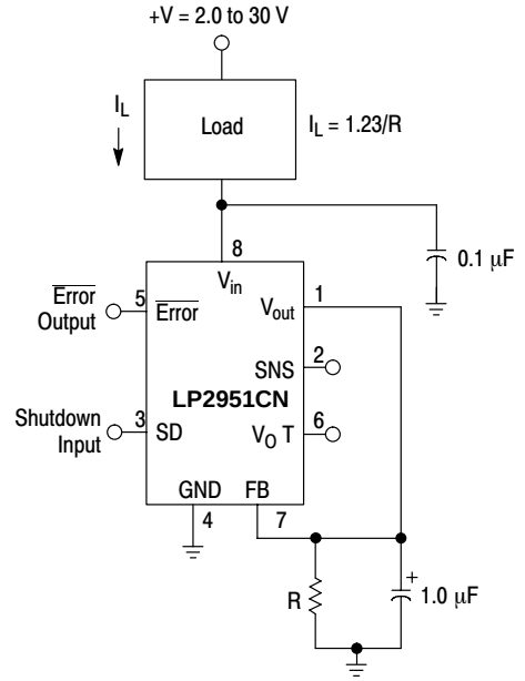
Figure 21. Low Drift Current Sink
