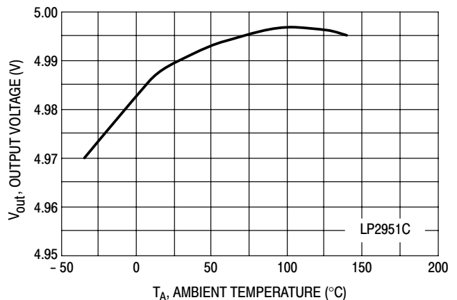
Figure 5. Output Voltage versus Temperature
