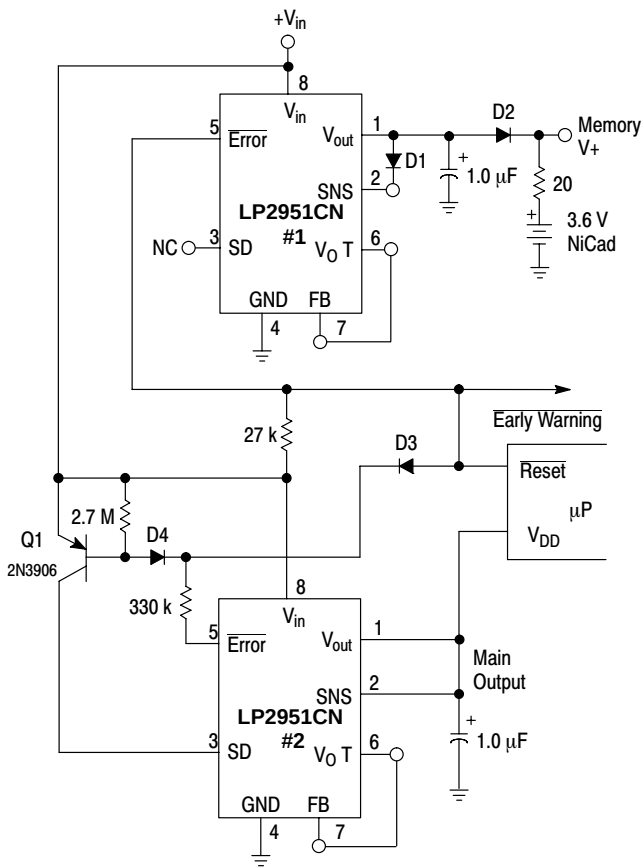
Figure 24. Regulator with Early Warning and Auxiliary Output
