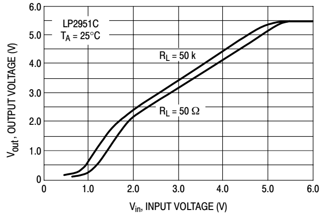
Figure 3. Dropout Characteristics
