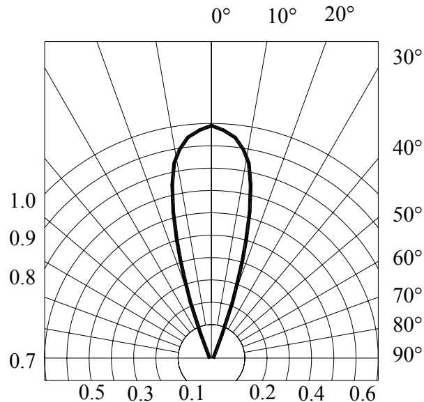
RADIATION DIAGRAM
