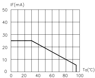
FIG.5 MAXIMUM FORWARD CURRENT VS. AMBIENT TEMPERATURE ( T_{j\text{max}}=105^{\circ}\text{C} )
