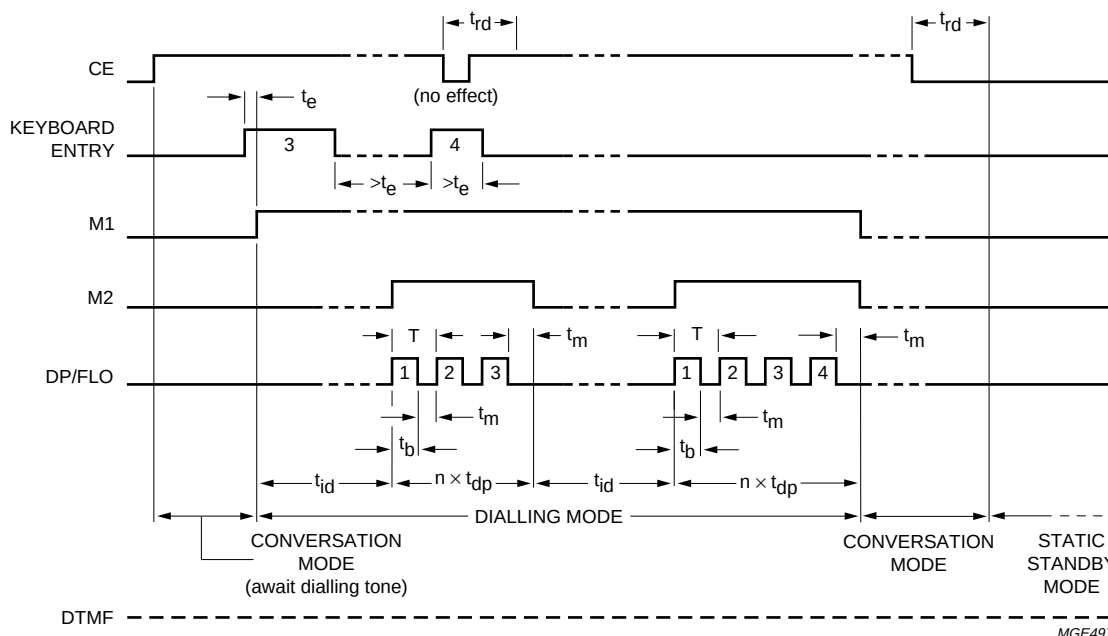
Fig.11 Timing diagram for pulse dialling ( \overline{\text{PD}}/\text{DTMF} = V_{SS} ).
