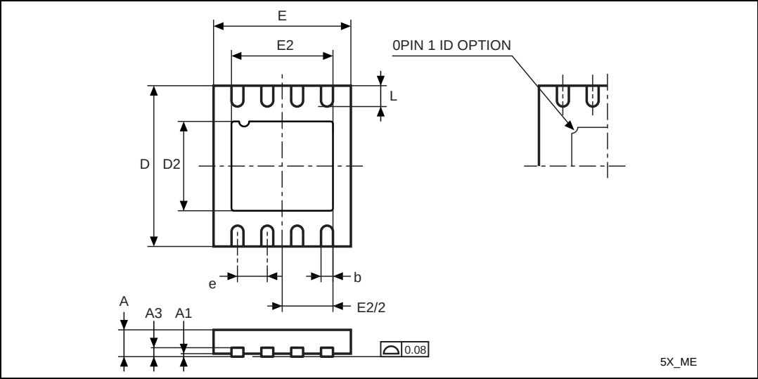
Figure 28. QFN8L (MLP8) 8-lead, quad flat package no lead, 6 × 5 mm, package outline
