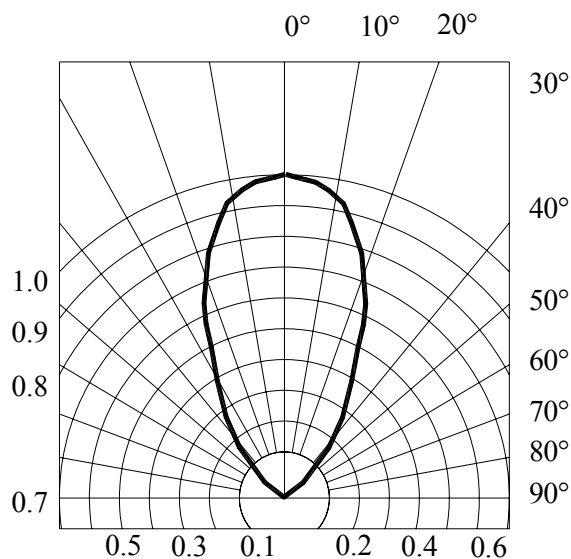
RADIATION DIAGRAM
