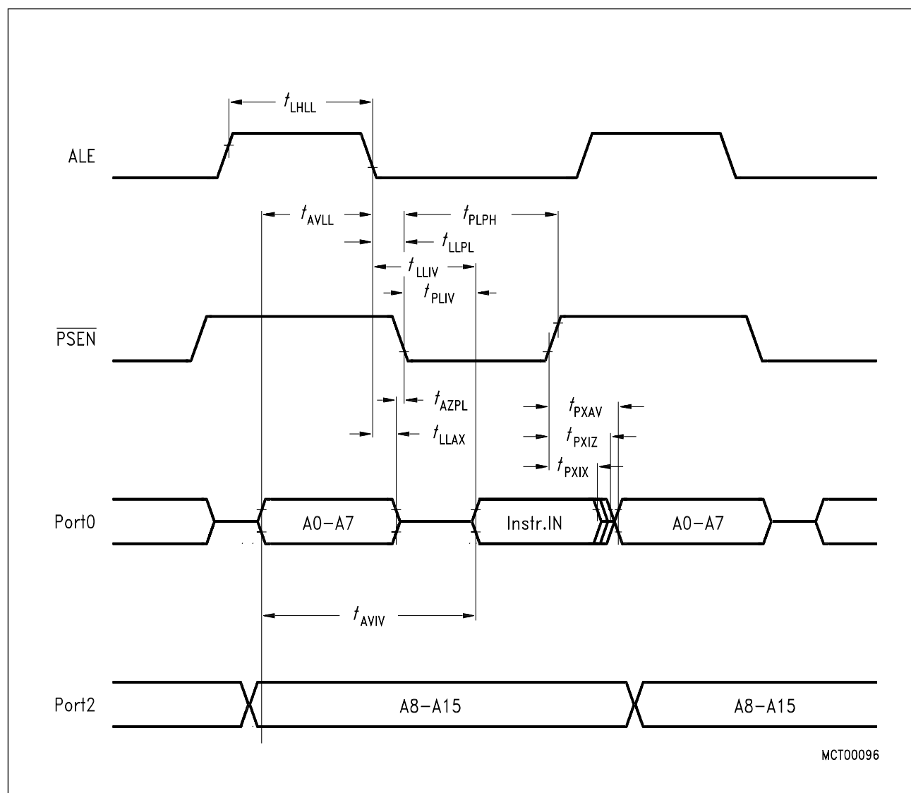
Figure 7 Program Memory Read Cycle
