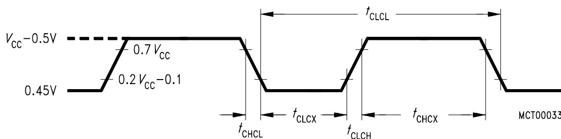
Figure 13 External Clock Cycle
